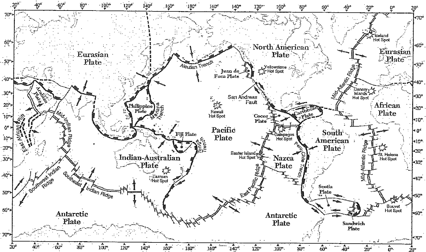
Tectonic Plates
