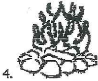
4. Radiation
