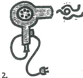
2. convection
