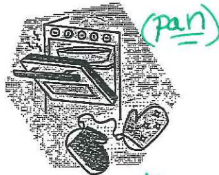
8. (pan) conduction
