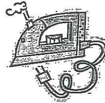
3. conduction
