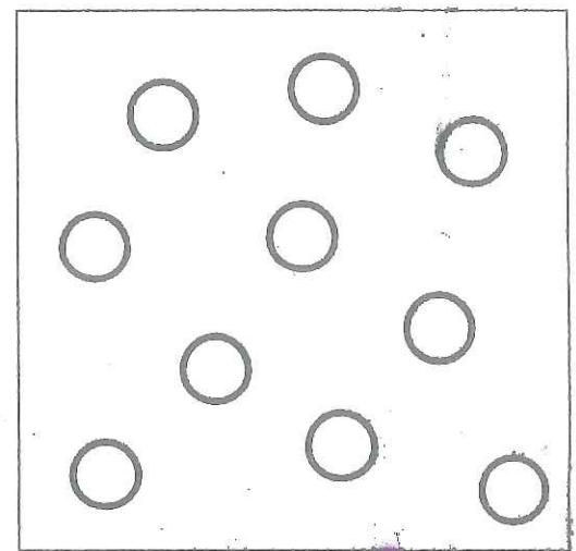
Gas
